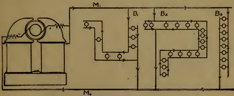
Figure 4 Typical constant potential system.
